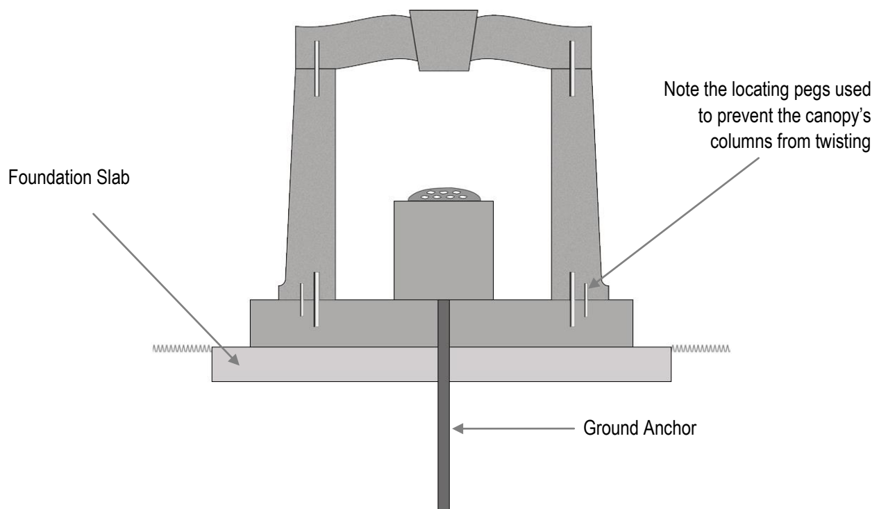
Fig 11 ~ A typical Canopy Set fixed using dowels, locating pegs and ground anchor
